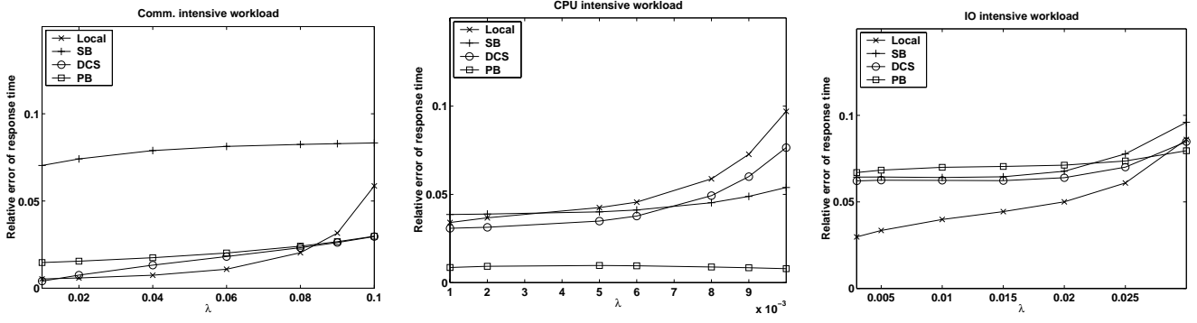
Figure 1: Validation Results.
