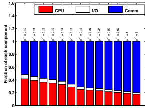
(e) Application Profile for SB (time unit is millisecond, \lambda = 0.006 )
