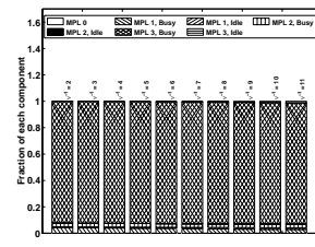
(c) System Profile at Maximum Utilization for PB (time unit is millisecond.)
