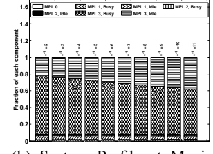
(b) System Profile at Maximum Utilization for SB (time unit is millisecond)
